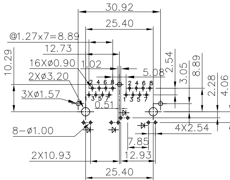
PC Board Layout Component Side Shown PC Board =1.60 mm
